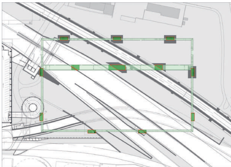
Fig. 1 Situation mit Neubau und darunter verlaufender Infrastruktur. Situation of the new building and the infrastructure running underneath it.
