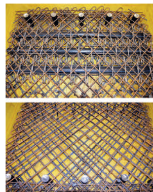
Rotated reinforcement layout with embedded ducts and without embedded ducts.
