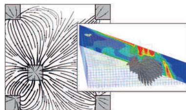
Visualization of shear flow in a thick transfer slab.
